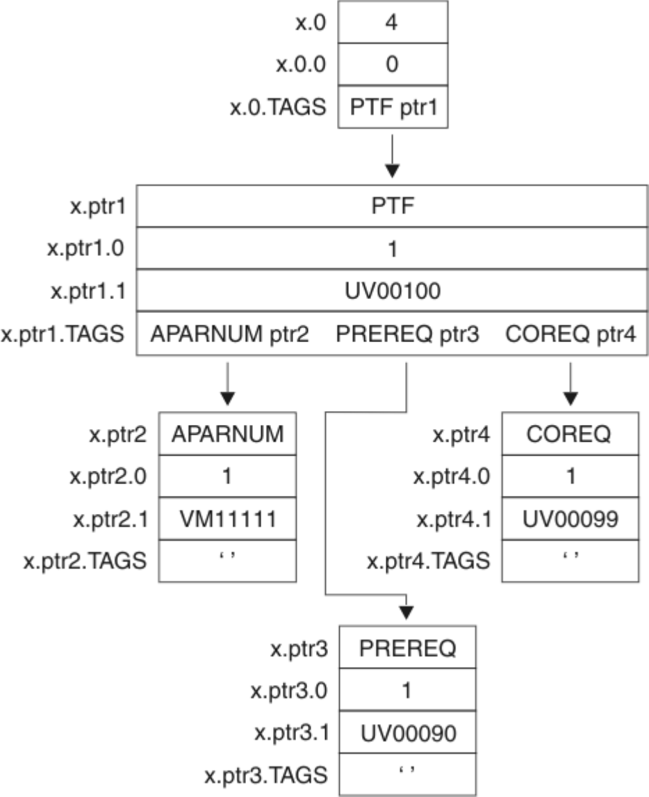
Figure 171. Tree Structure Format
