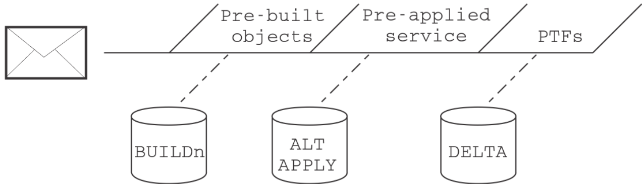
Figure 66. Preventive Service Files
