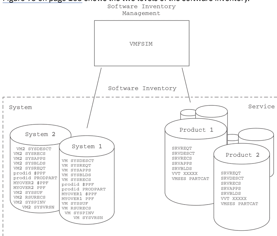
Figure 93. Software inventory files in the VMSES/E database
