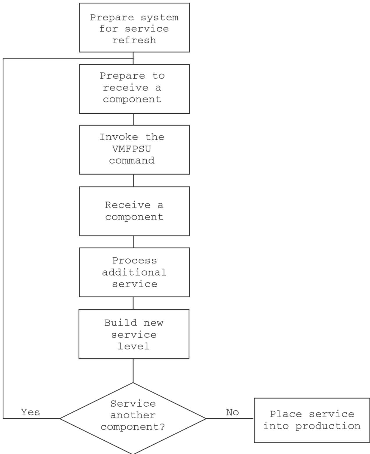
Figure 67. Service application flowchart using the product service upgrade procedure
