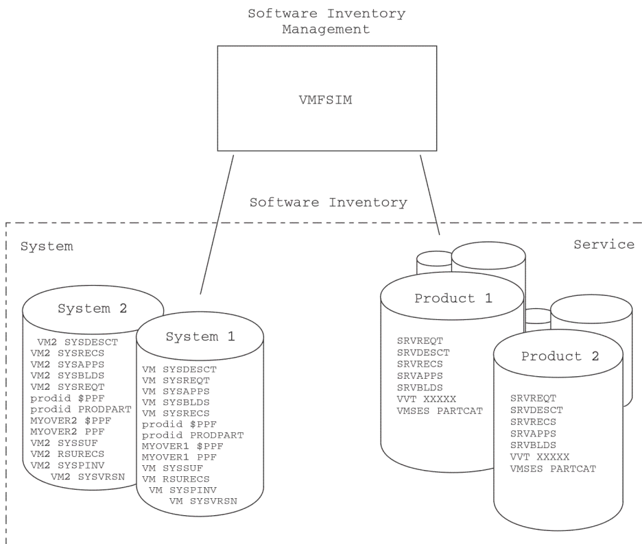
Figure 4. The system-level and service-level software inventories
