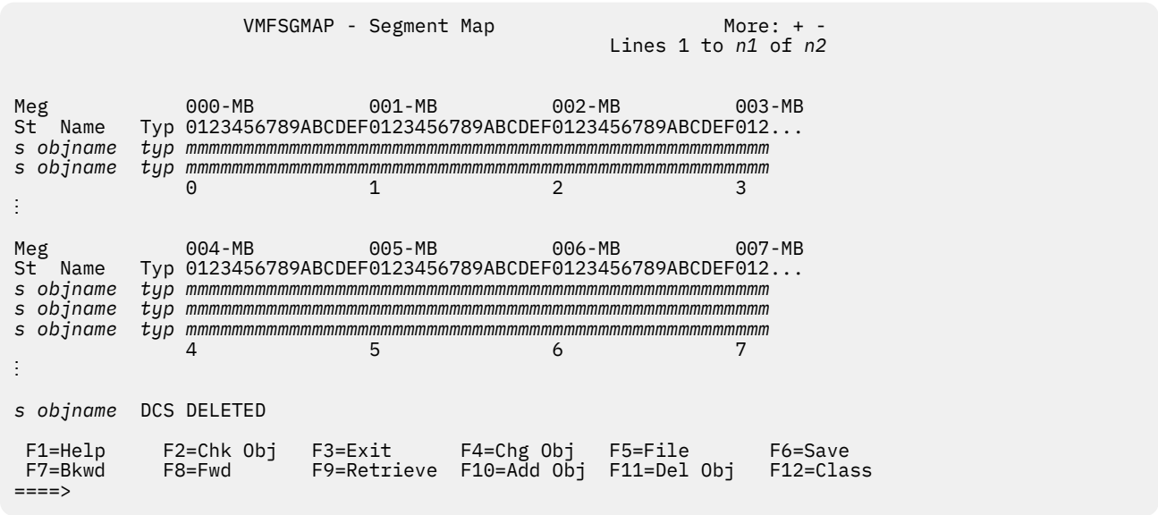
Figure 164. VMFSGMAP Segment Map Panel with Status Codes
