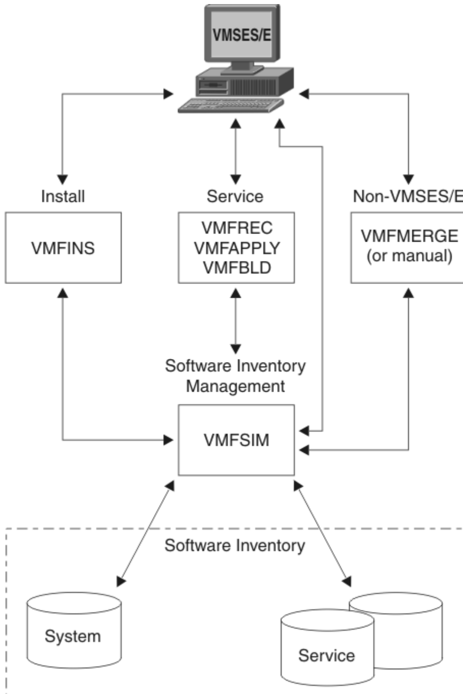
Figure 141. VMSES/E - Reference Information
