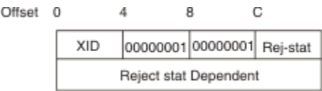
Figure 97. Structure of an RPC Rejected Reply Message
