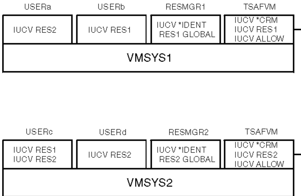
Figure 141. TSF Collection with Authorized Global Resource Managers and User Programs
