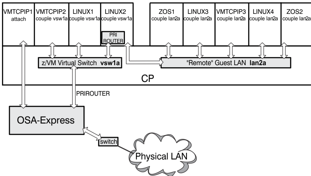
Figure 23. Virtual Switch with Remote Guest LAN
