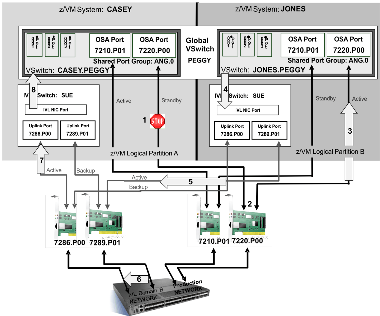
Figure 59. LAG Port Controller Take-Over Sequence
