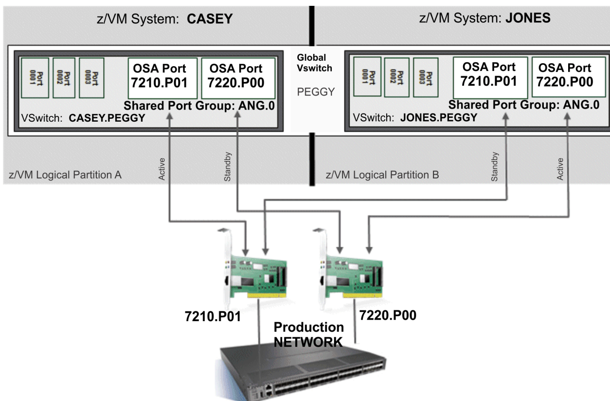
Figure 57. Global VSwitch PEGGY with shared port group ANG
