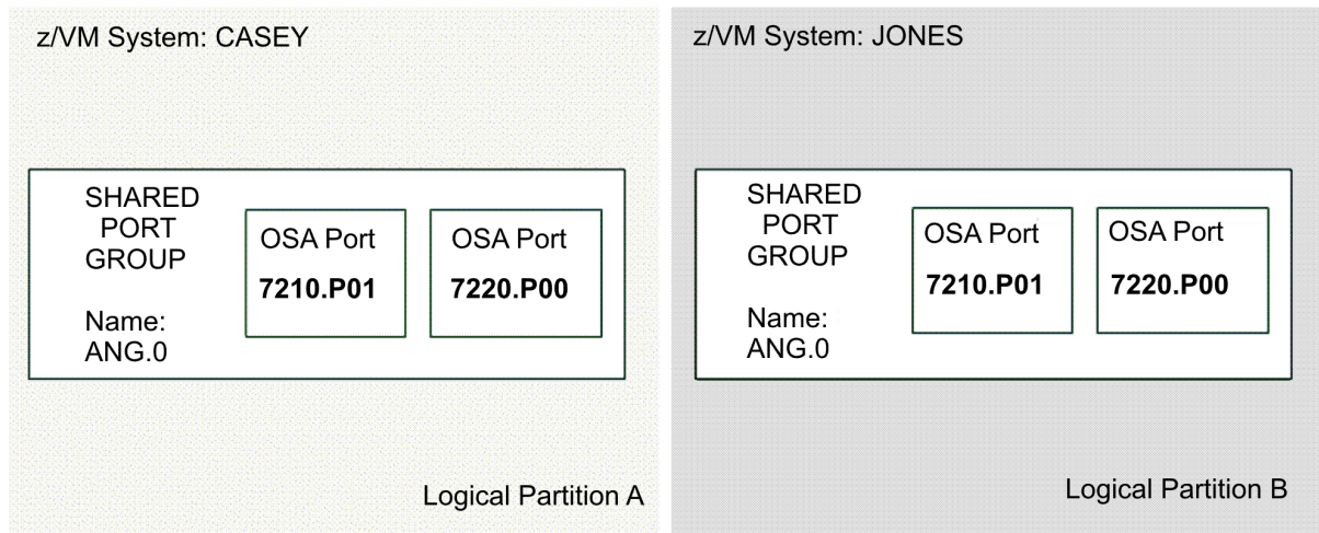
Figure 45. Shared Port Group ANG
