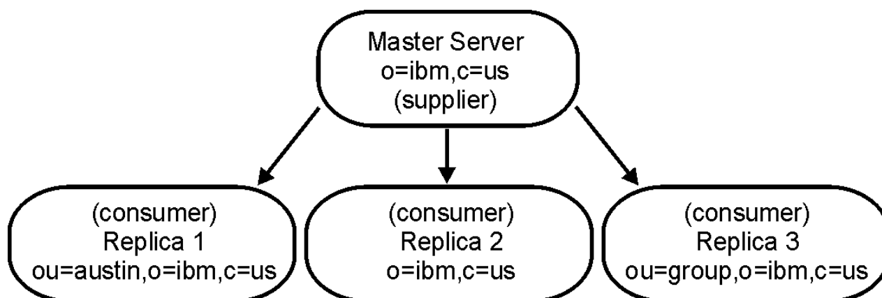
Figure 37. Master-replica replication
