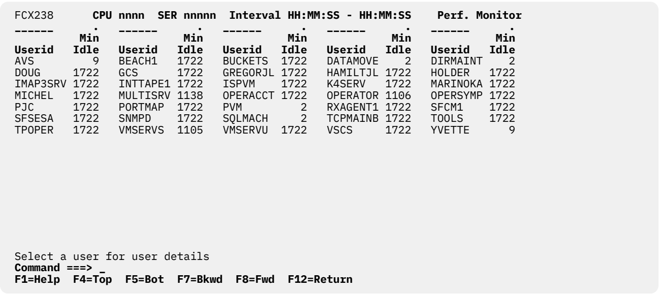
Figure 132. Layout of Idle Users Screen (FCX238)
