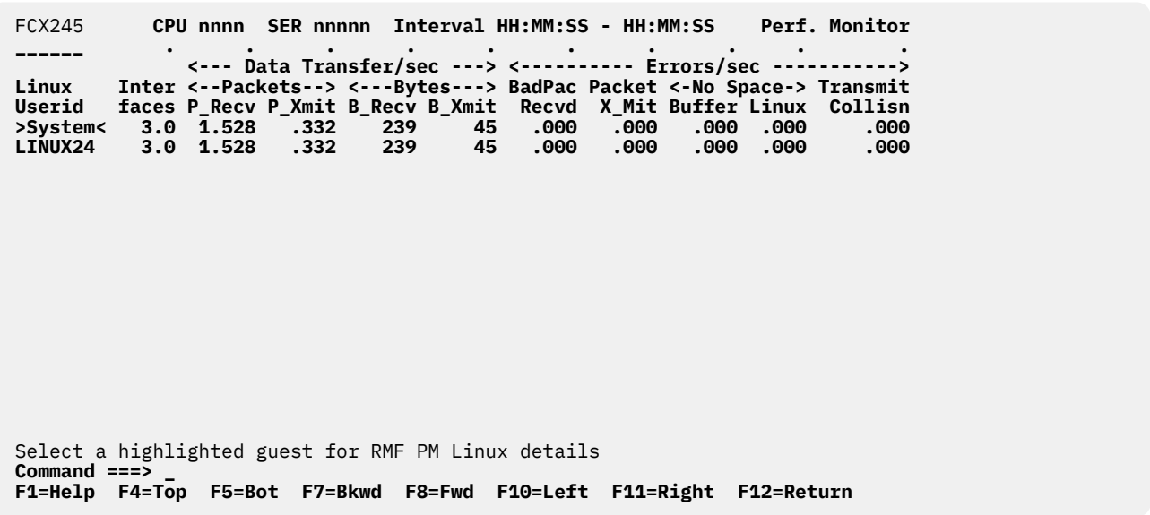
Figure 139. Layout of General Linux Networking Activity Screen (FCX245)
