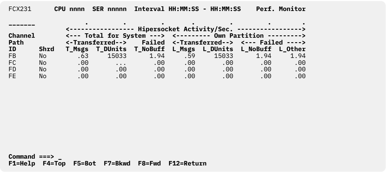
Figure 125. Layout of Hipersocket Channel Activity Screen (FCX231)
