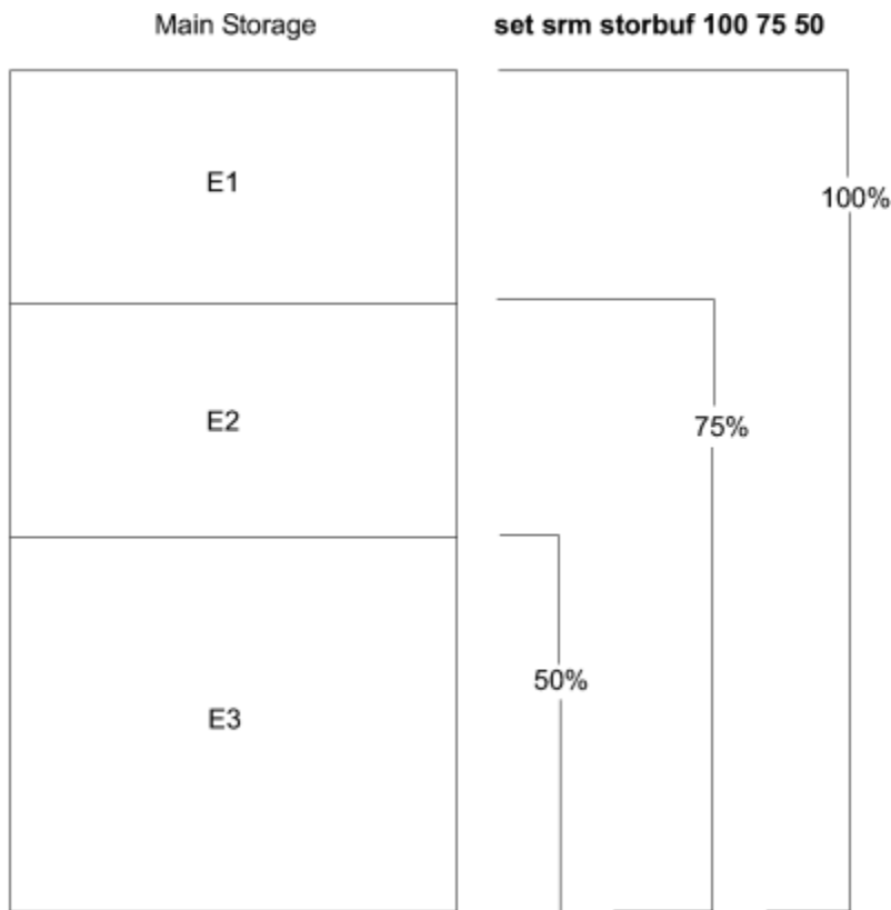
Figure 10. How the SET SRM STORBUF Command Works
