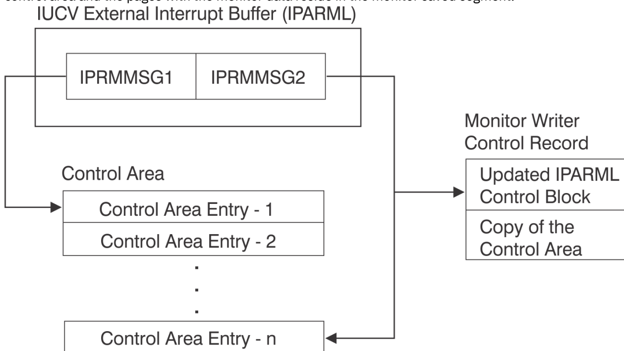
Figure 16. Putting *MONITOR Data into the MONWRITE Control Record
