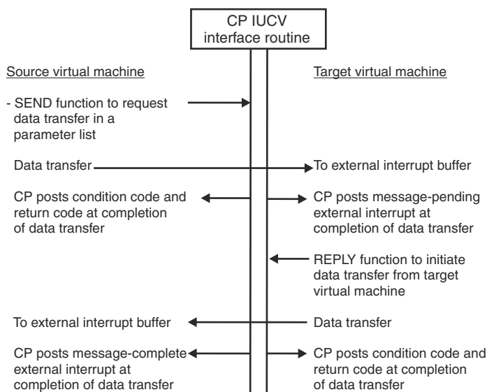
Figure 21. Flow of the IUCV SEND/REPLY Protocol
