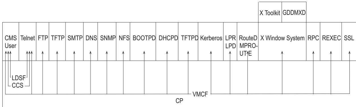
Figure 3. The TCP/IP Layered Architecture for VM
