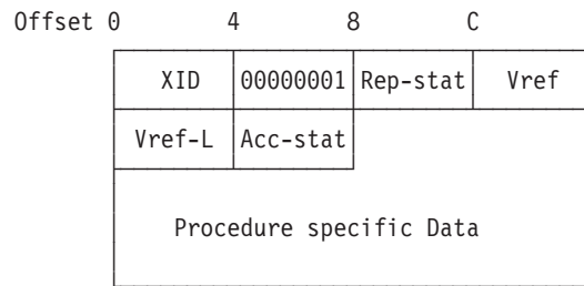
Figure 83. Structure of an RPC Accepted Reply Message
