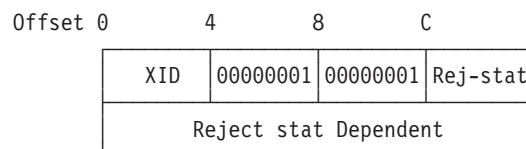
Figure 84. Structure of an RPC Rejected Reply Message
