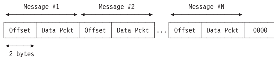
Figure 99. PCCA Block Structure
