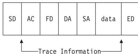
Figure 103. Common Layout of a Token-Ring Packet
