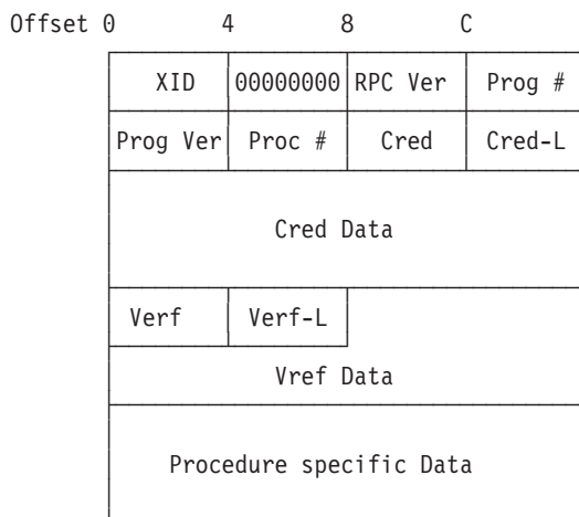
Figure 82. RPC Call Message Structure
