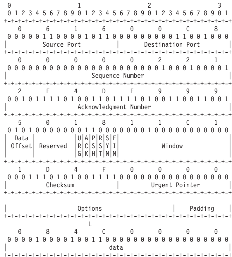
Figure 108. TCP Header Format
