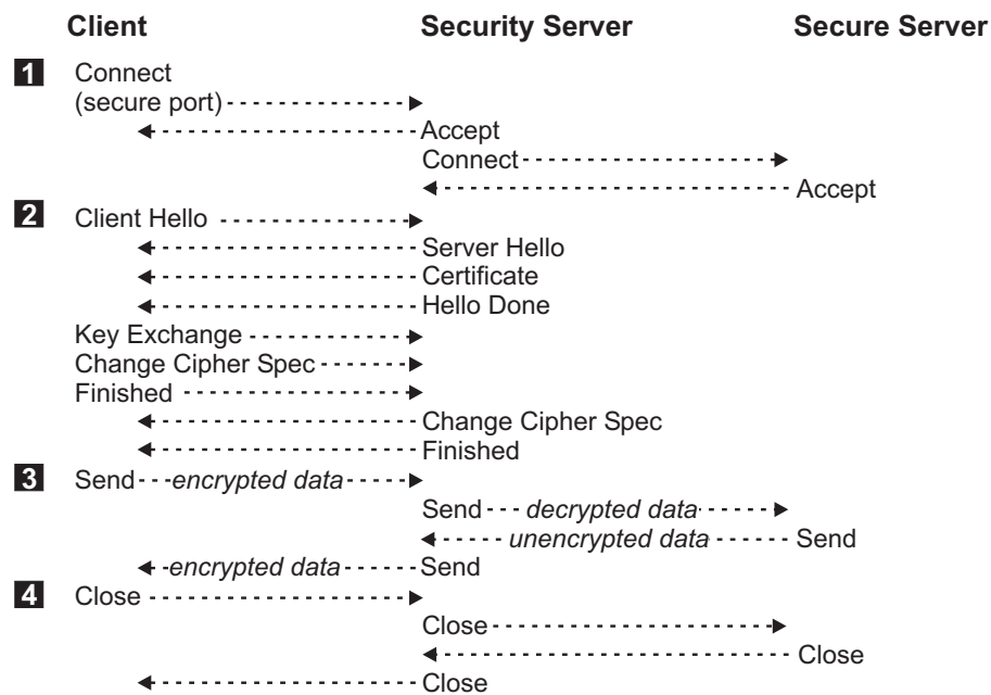
Figure 89. SSL processing flow
