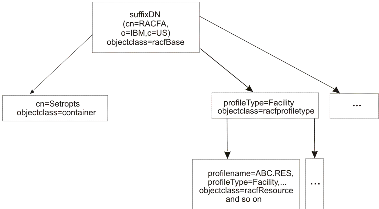
Figure 19. RACF namespace hierarchy (Part 2 of 2)
