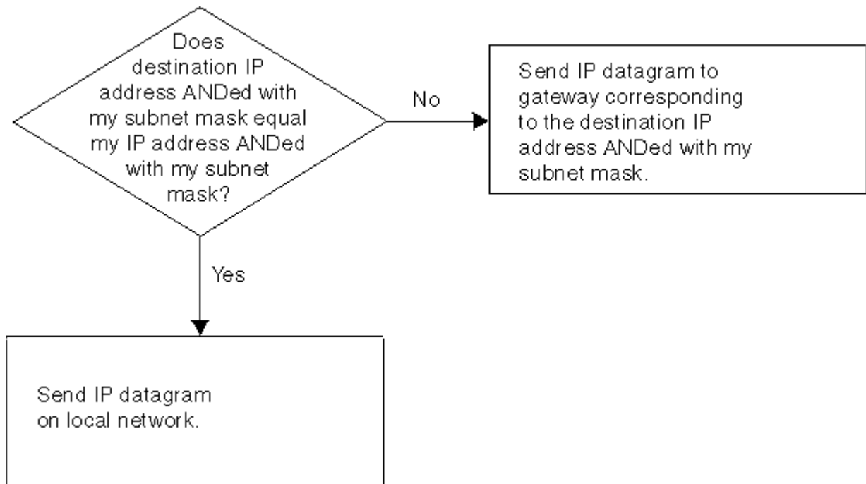
Figure 16. Routing Algorithm with Subnets
