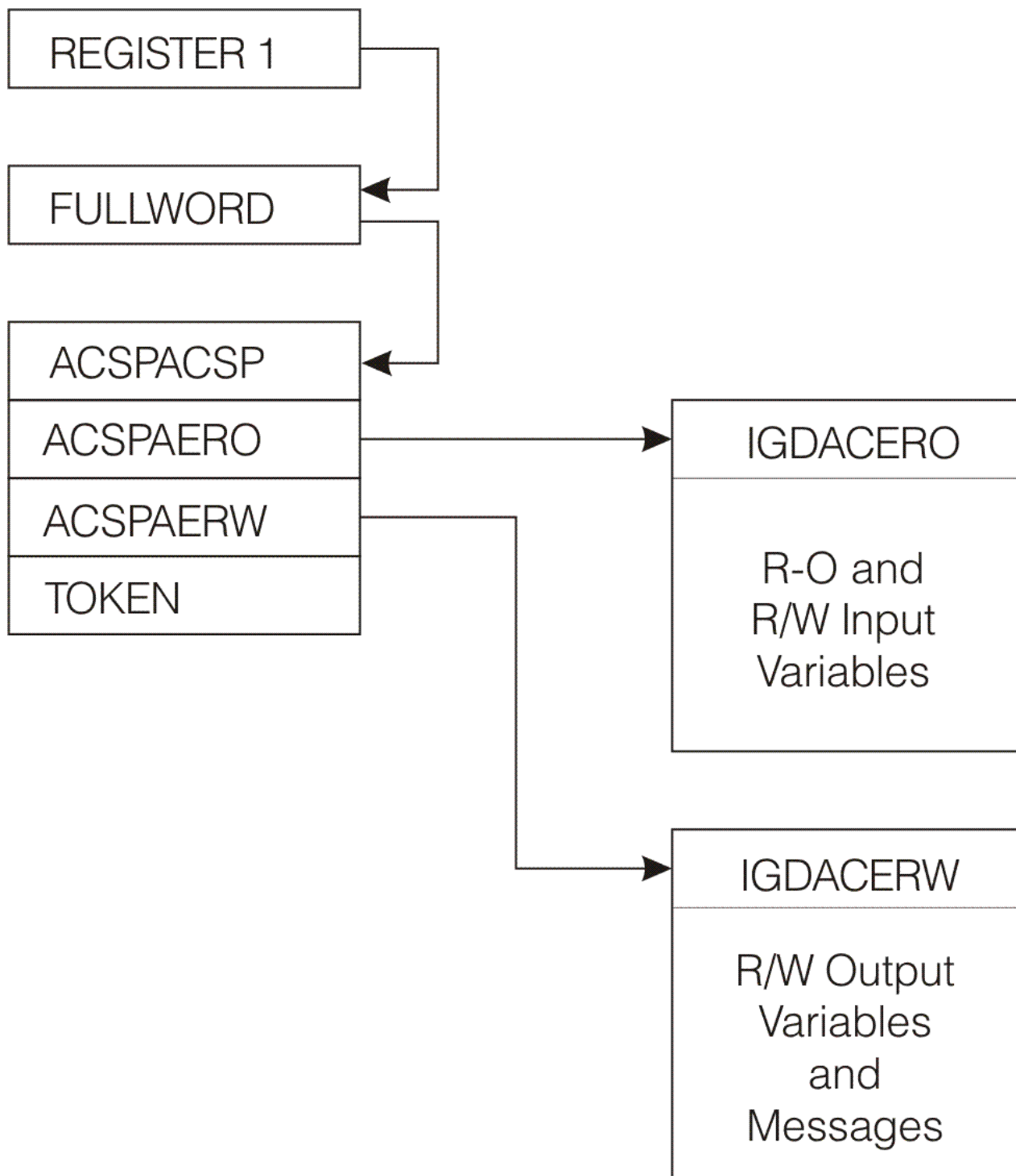
Figure 111. Parameter Structure for the ACS Interface Routine
