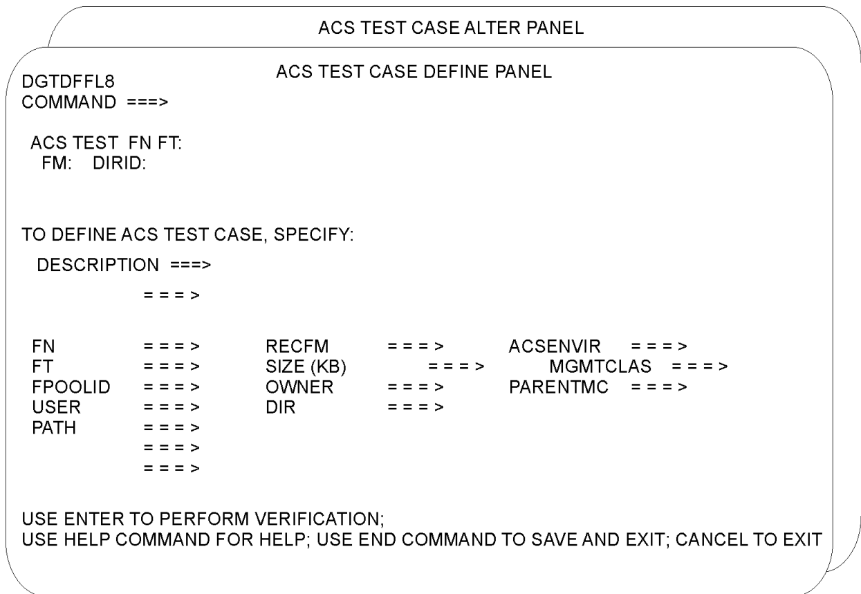
Figure 40. ACS Test Case Define/Alter Panel for DFSMS/VM
